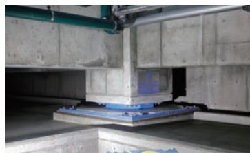
Structure fitted with seismic isolators
